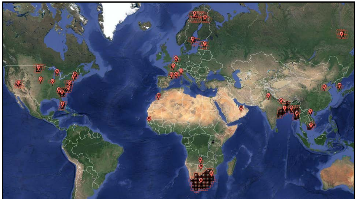
Figure 4: Map of the 39 regions with the 366 MGRS tiles footprint (black) and the 360 Landsat WRS-2 path-row (red). Get an interactive map here .
